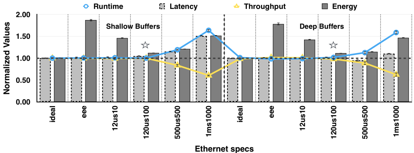
Fig. 2. Runtime, Latency, Throughput and Energy values for Packet Coalescing combined with RED and ECN
