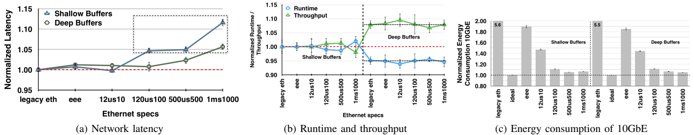
Fig. 1. Packet coalescing impact considering different buffer sizes
