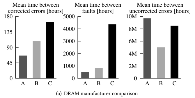
(a) DRAM manufacturer comparison
