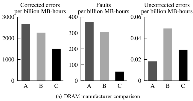
(a) DRAM manufacturer comparison
