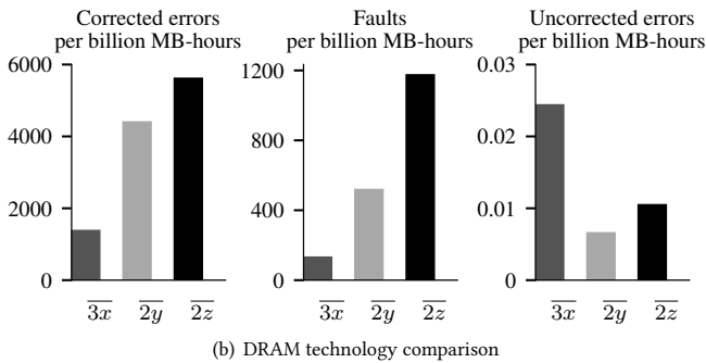
(b) DRAM technology comparison
